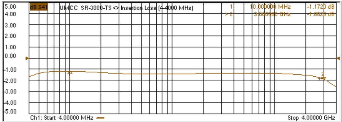
-Insertion Loss (4-4000MHz)
