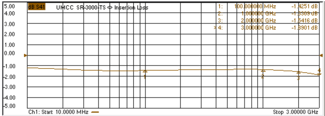
-Insertion Loss
