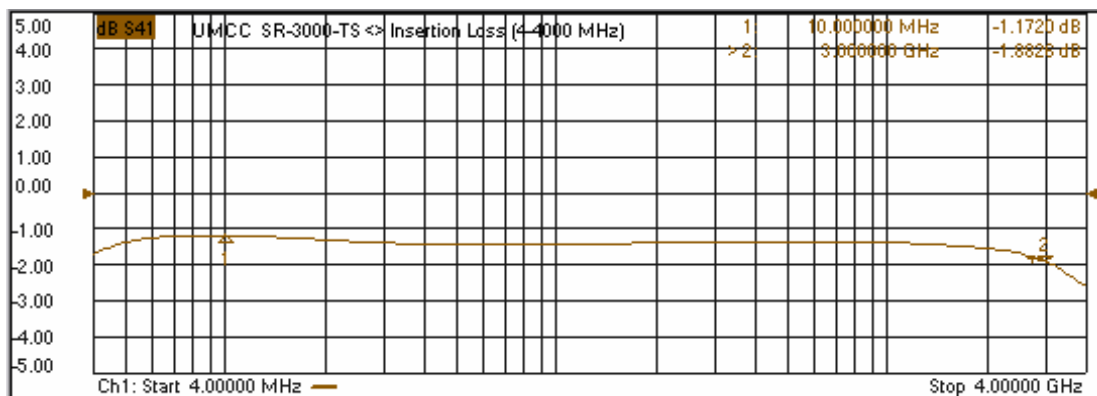
-Insertion Loss (4-4000MHz)
