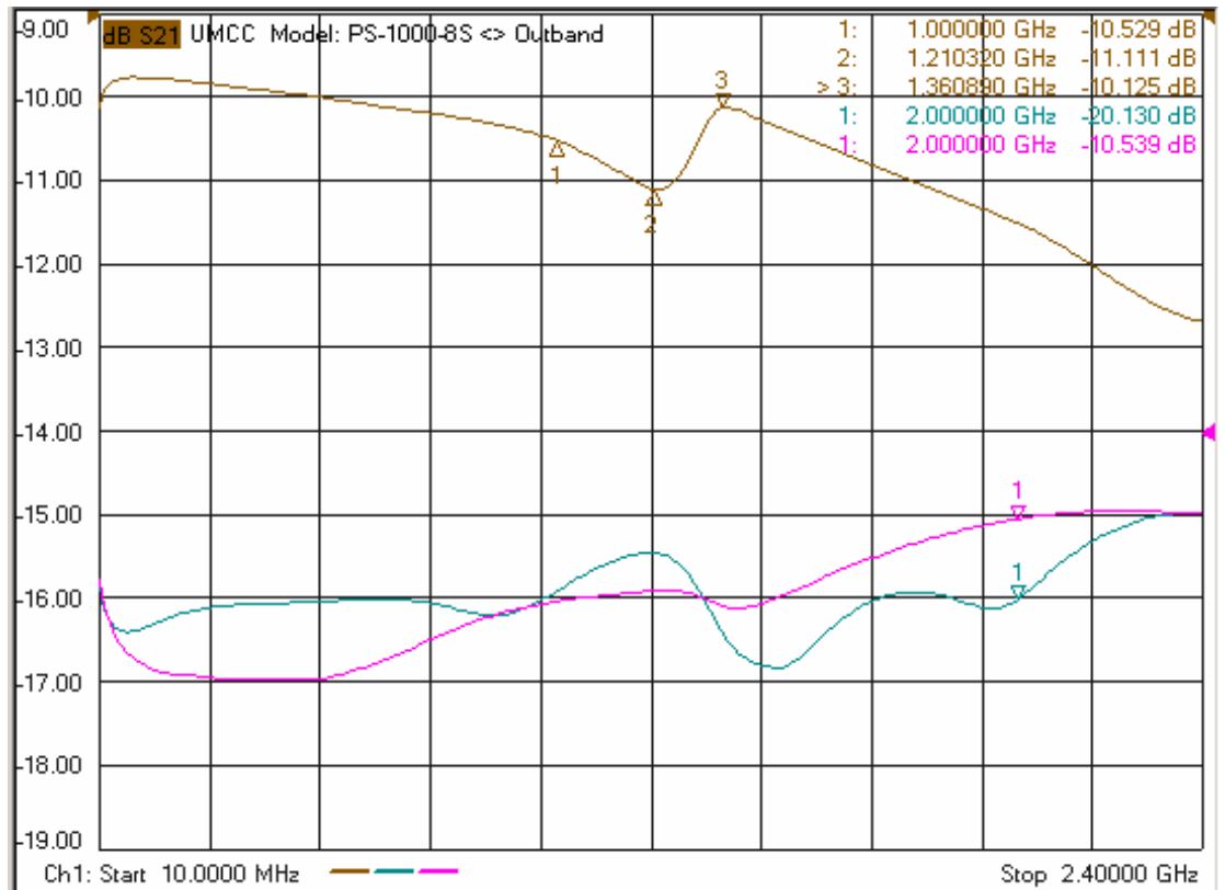
- Out Band Frequency Response
