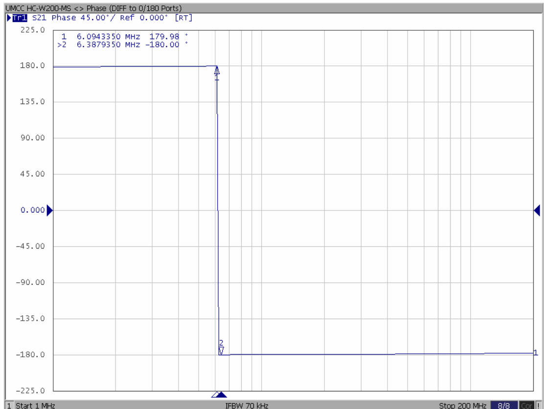
-Phase Error DIFF to 0/180 Ports
