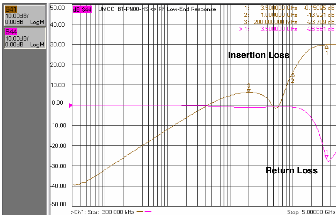
- Out-Band Low-End Freq. Response
