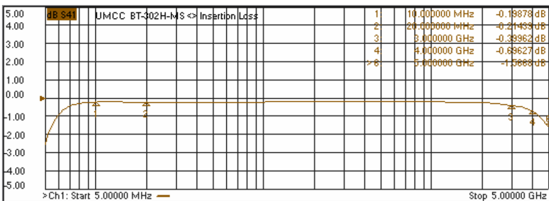
"Out-Band Response" (5MHz - 5GHz)
