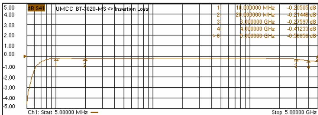
"Out-Band Respose" (5MHz - 5GHz)
