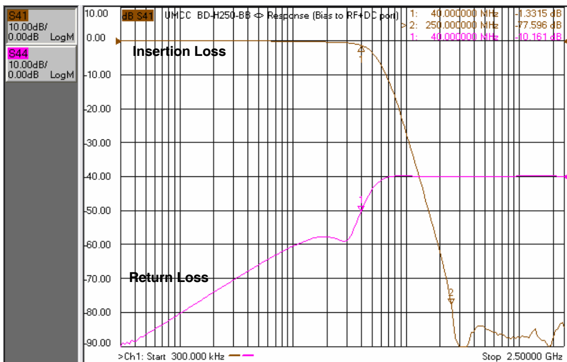
- Bias Freq. Response (Bias to RF+DC)
