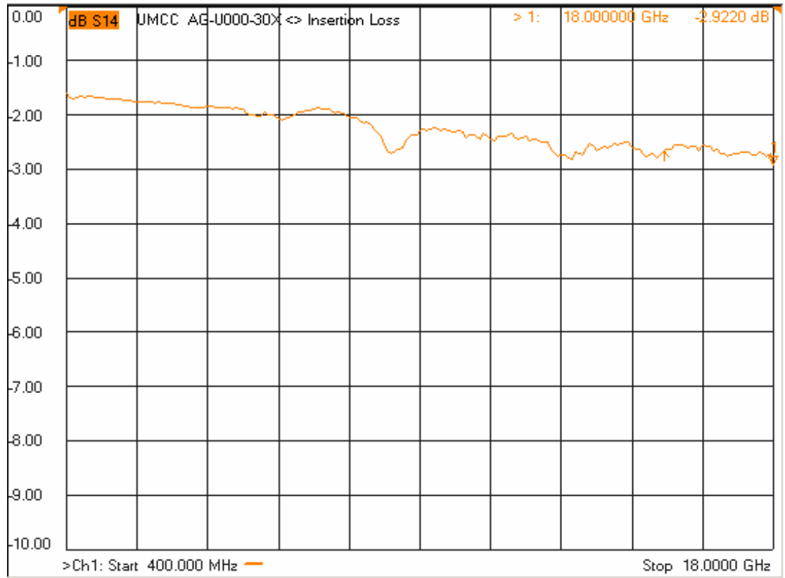
- Insertion Loss
