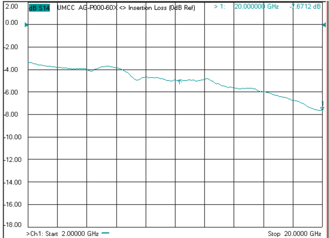
- Insertion Loss
