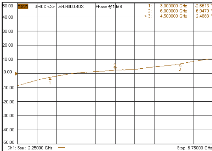
Phase Shift @ 10dB Attn.
